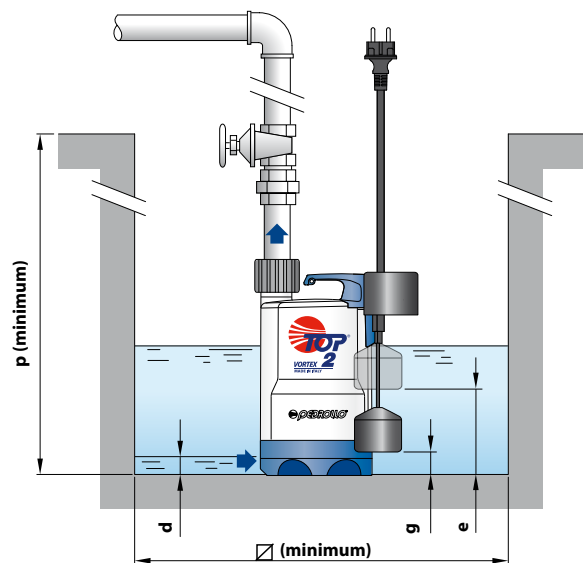
Typical installation
