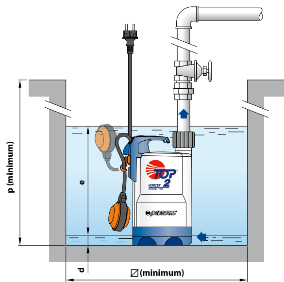
Typical installation
