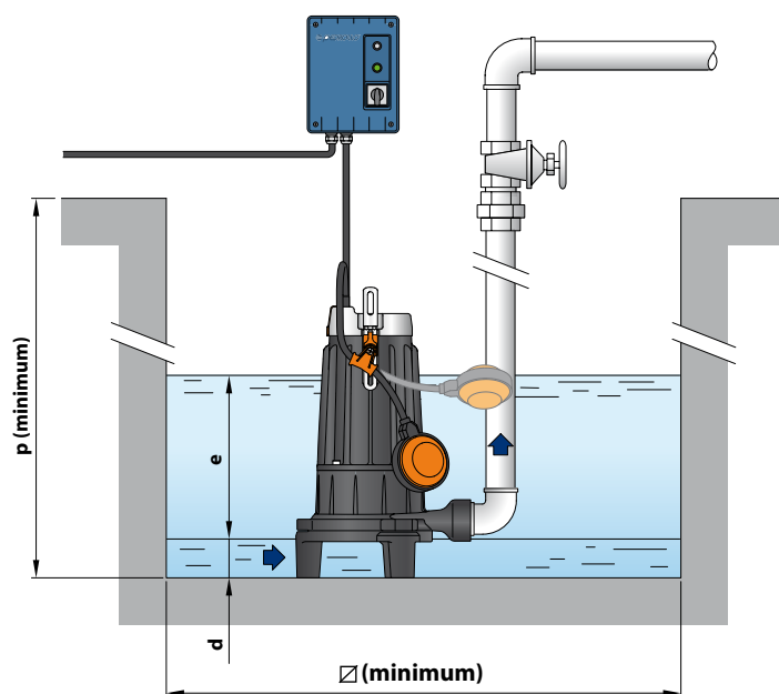
Typical installation
