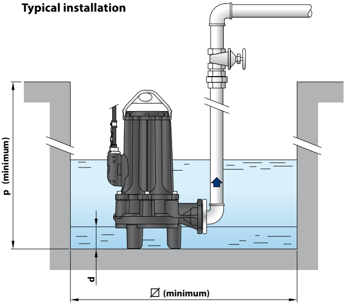
Typical installation
