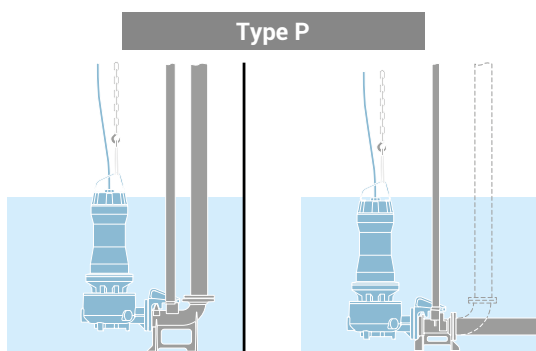
Installation with coupling device with vertical (DAC V) or horizontal (DAC H) discharge Flushing valve (FLX) admitted
