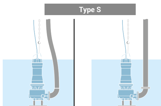
Free installation with base (KBS) Flushing valve (FLX) admitted
