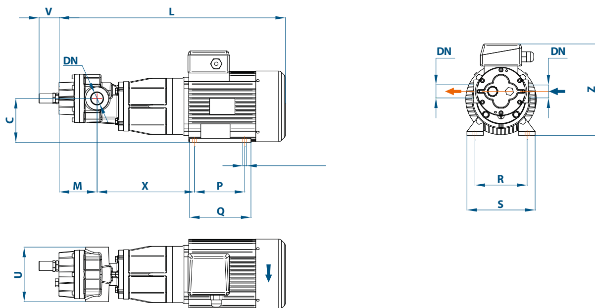
Fig. 409 - BFC dimensional drawing with motor
