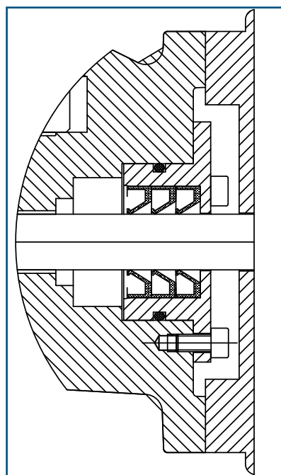
Fig. 406 – Lip seal
